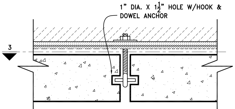
3 HORIZONTAL SECTION
