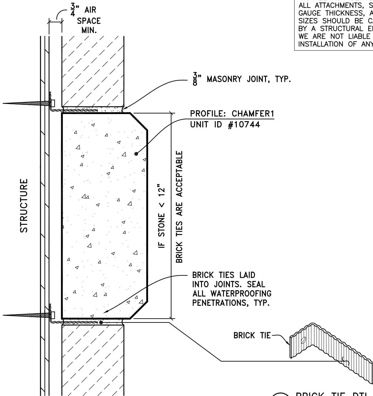
2 BRICK TIE DTL. GALVANIZED OR BETTER
