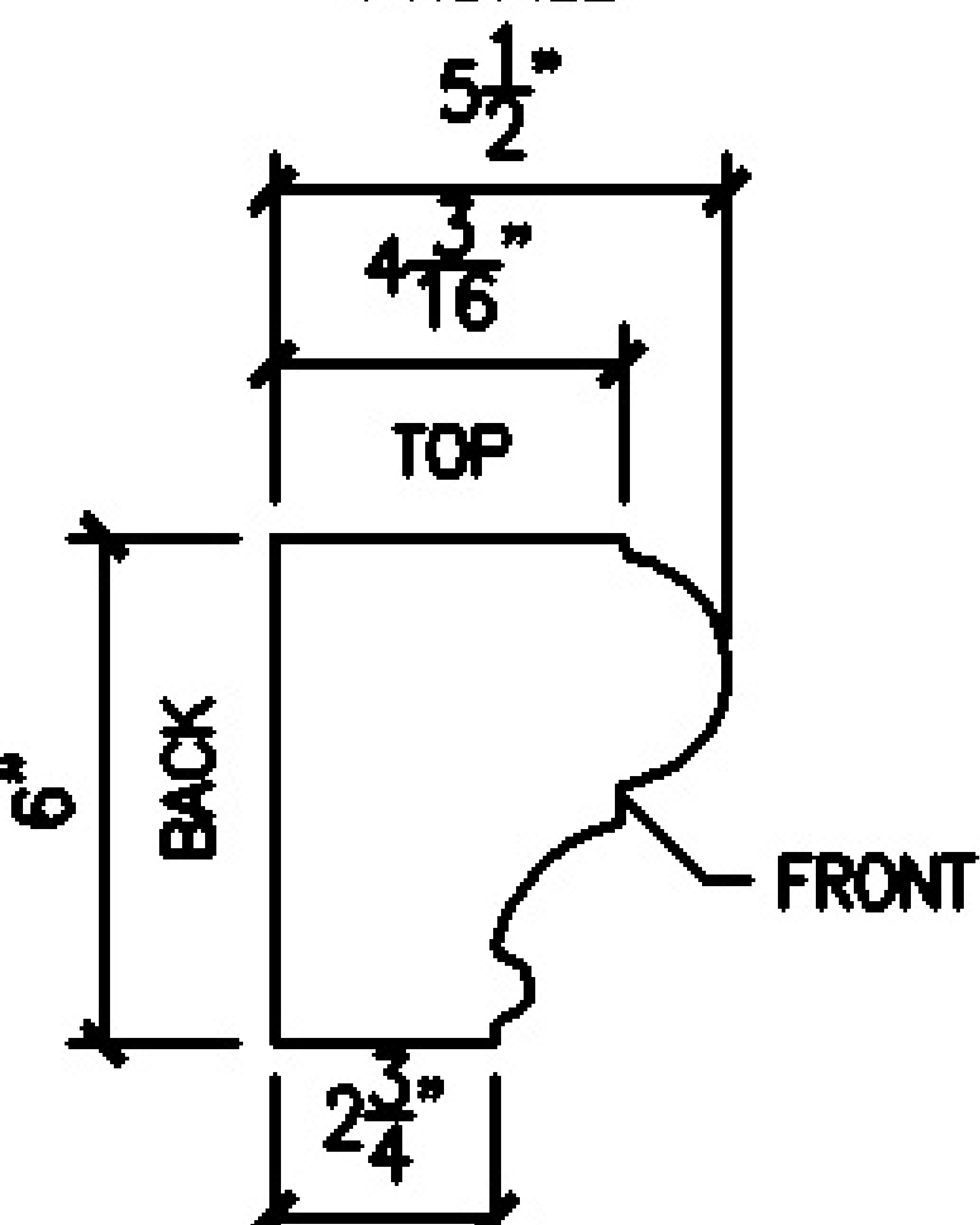
MARCUS3 PROFILE
