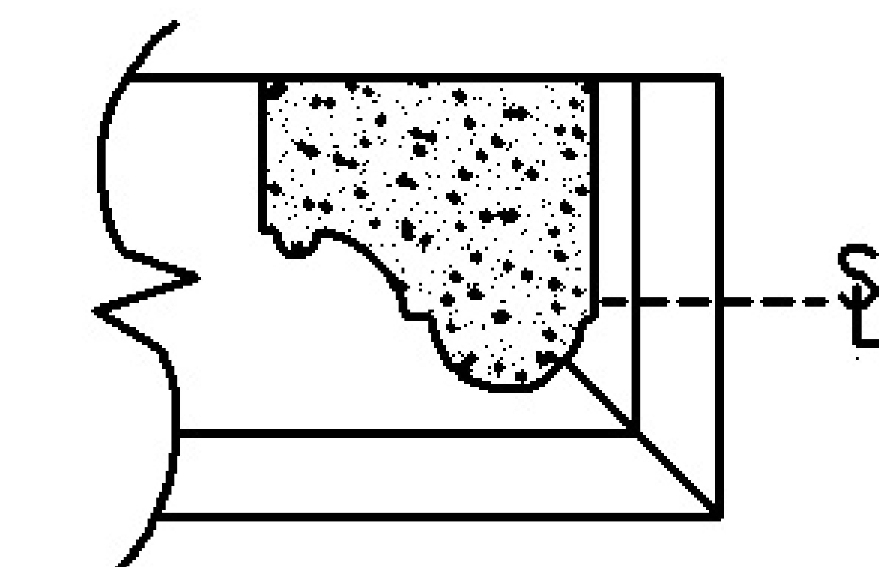
2 SECTION LEG AT SILL
