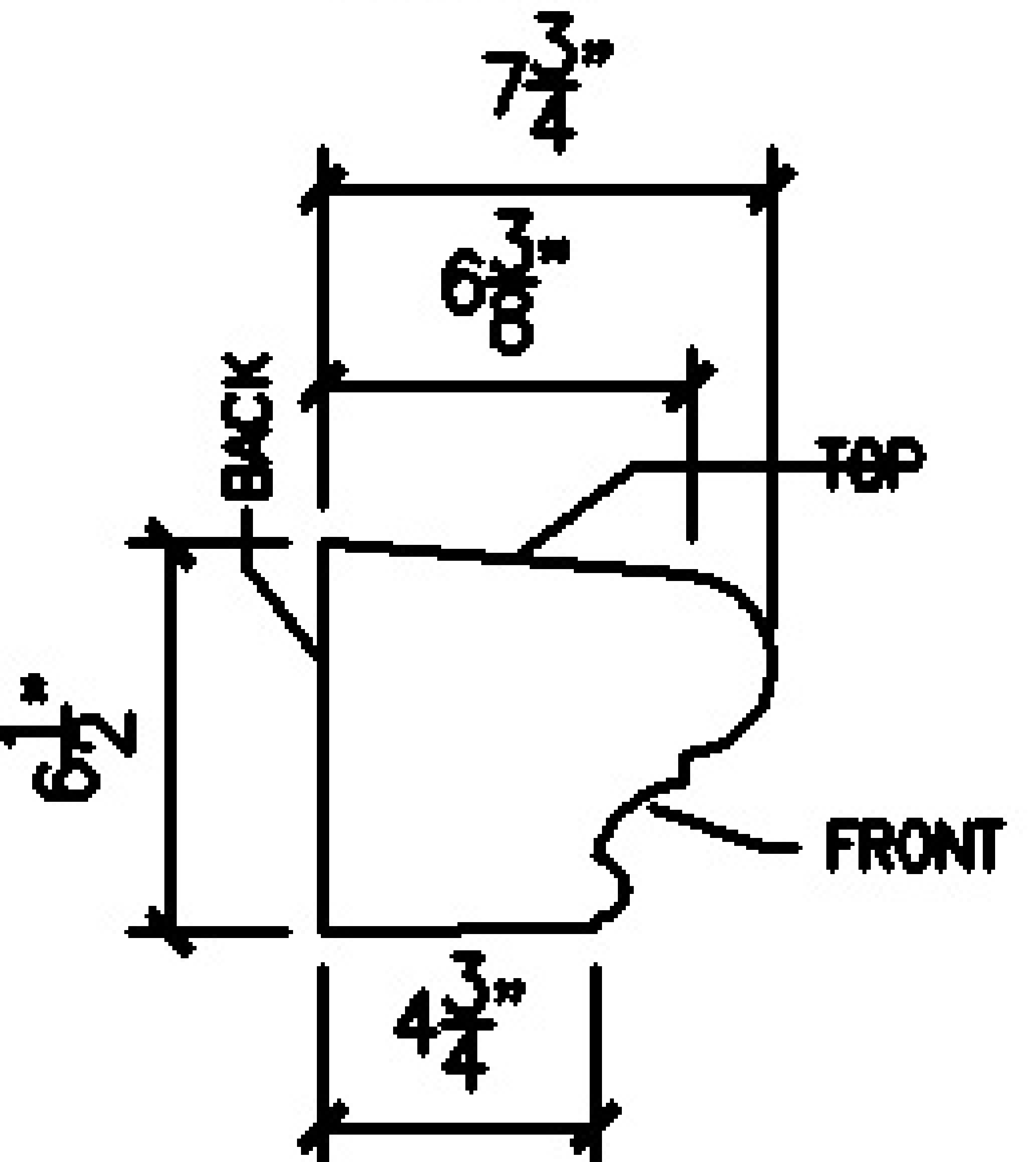
MARCUSSLOPE1 PROFILE
