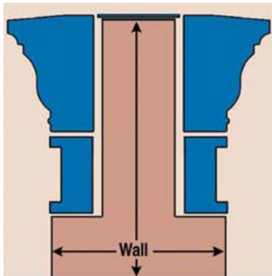
Mortar Filled
