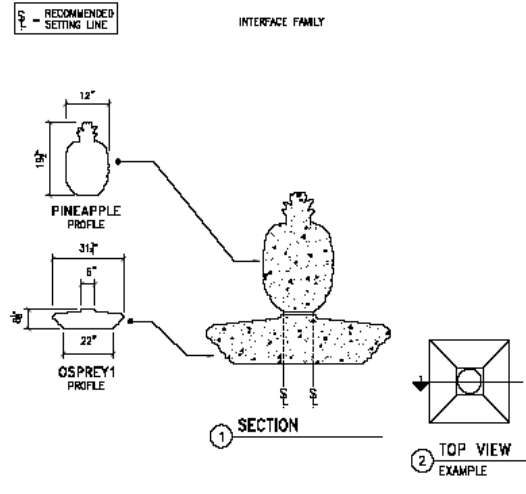
Pineapple Finial Cap Osprey1 Profile Setting Bed 12 inches
