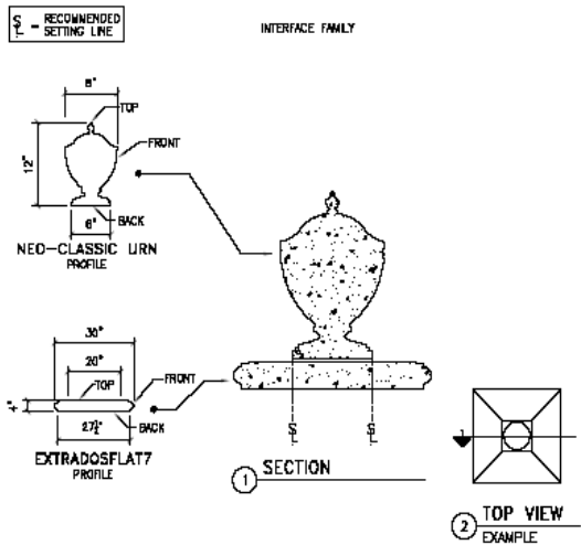
Neo-Classic Urn Finial Cap Extradoflat7 Profile Setting Bed 6 inches
