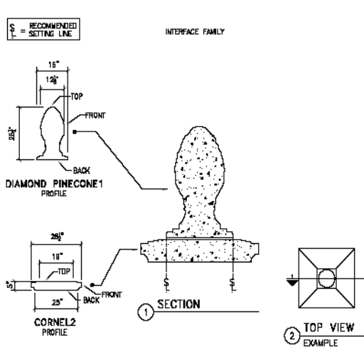
Diamond Pinecone1 Finial Cap Cornel2 Profile Setting Bed 16 inches
