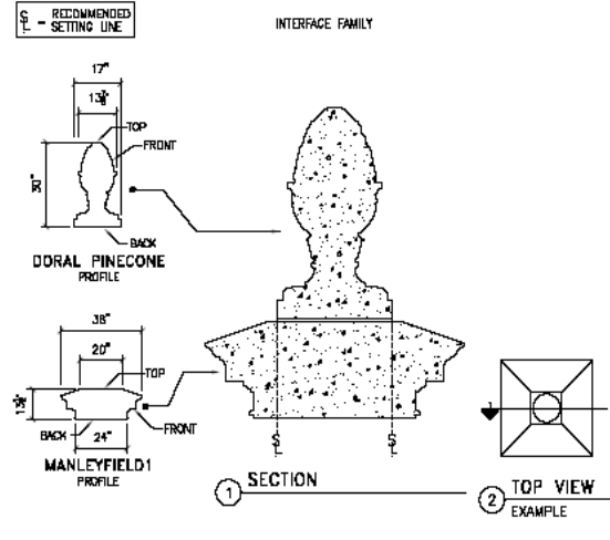
Doral Pinecone Finial Cap Manleyfield1 Profile Setting Bed 17 inches
