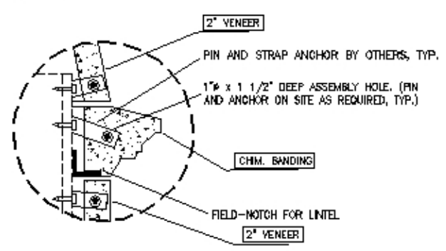
J CHIMNEY & VENEER PANELS SCALE: 1" = 1'-0"
