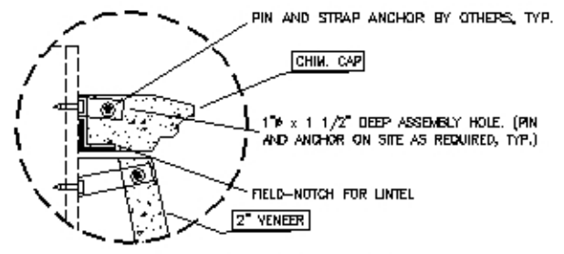
J CHIMNEY & VENEER PANELS SCALE: 1" = 1'-0"
