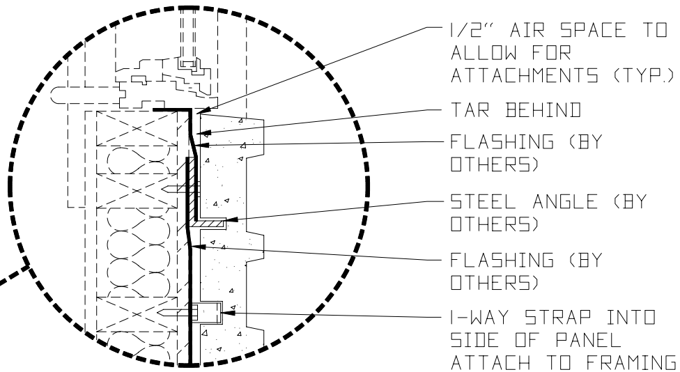
DETAIL VIEW
