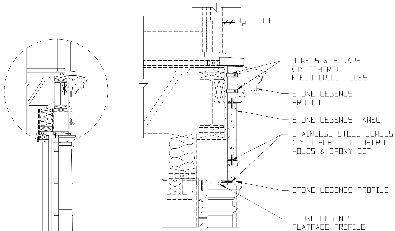
ENLARGED VIEW VERTICAL SECTION
