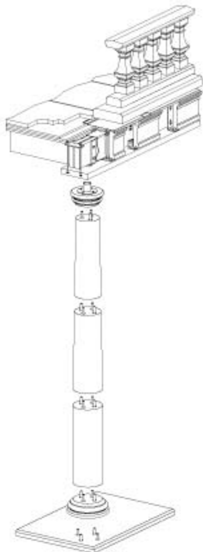
1 Column Assembly Exploded View
