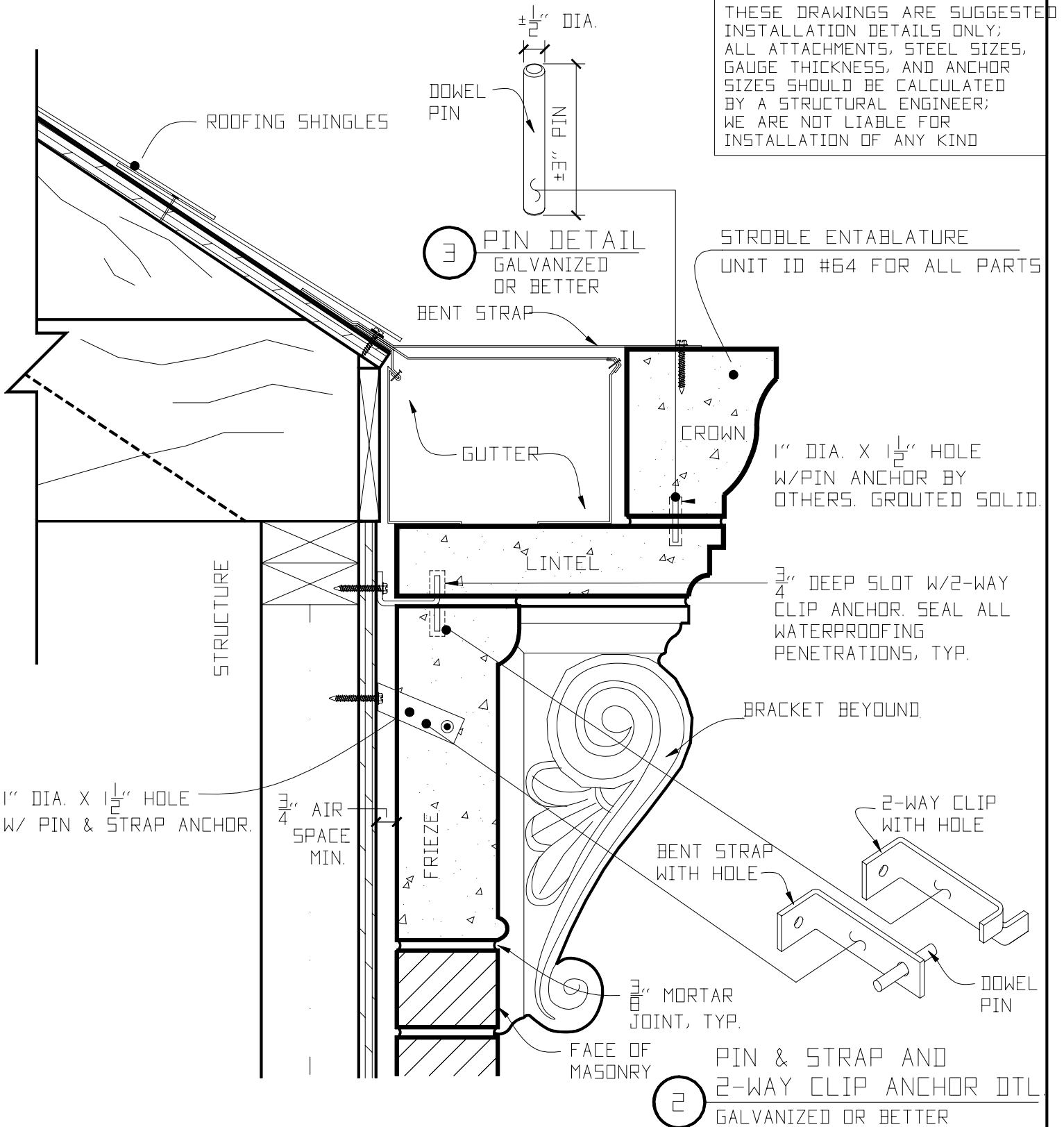
1 CAST STONE ENTABLATURE & GUTTER ATTACHMENT TO MASONRY VENEER WITH PIN & STAP ANCHOR AND 2-WAY STRAP ANCHOR
