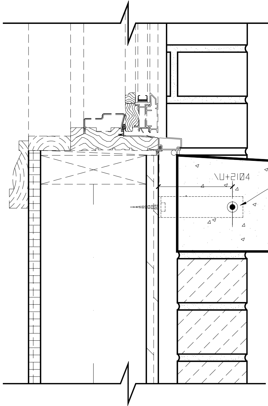
1 ATTACHMENT OF CAST STONE SILL TO BRICK WITH PIN & STRAP
