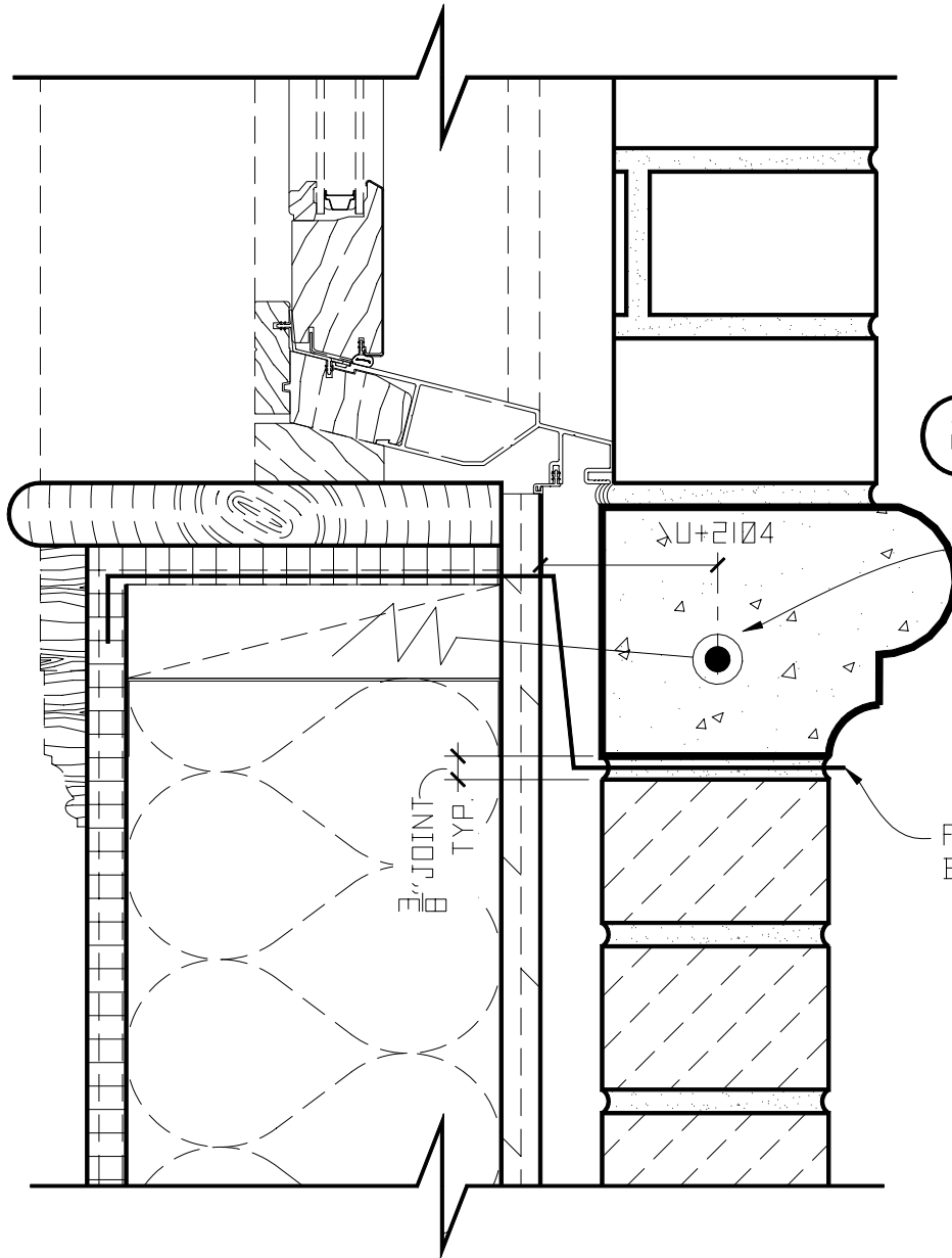
1 TYPICAL CAST STONE SILL DETAIL TO WITH PIN & WIRE BRICK
